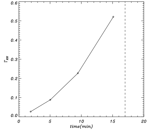
FIG. 15.— Normalized maximum KH growth rate, \Gamma_{KH} , as a function of time for the simulation shown in Figure 14. The dashed line corresponds to the time estimation of the onset of the KHI from the simulations.
