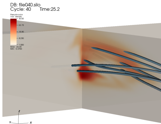
FIG. 16.— Same as in Figure 14 but for N_t = 4.3 .
