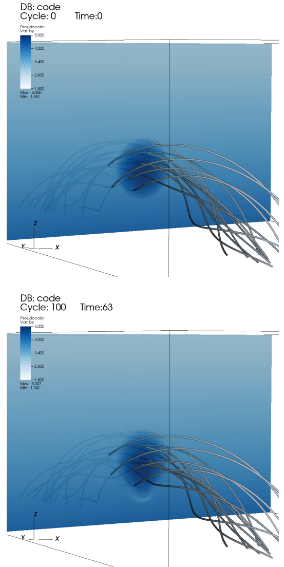
FIG. 2.— Snapshot of the flux rope configuration for N_t = 8.5 (strong twist). The B_y component of the magnetic field is plotted at the central plane together with some specific magnetic field lines. The upper panel corresponds to the test case without the prominence enhancement, while in the lower panel the dense prominence inside the flux rope is present (but not visible in this plot).
