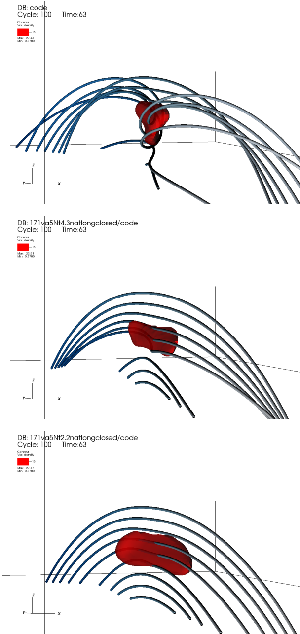
FIG. 4.— Snapshots of the flux rope configuration plus the prominence at the same instant for the cases N_t = 8.5 (top panel), 4.3 (middle panel), and 2.2 (bottom panel). The KHI is absent here because the spatial resolution is not high enough (600 km).
