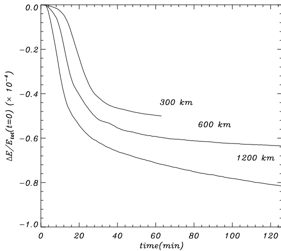
FIG. 9.— Change in total energy for different grid resolutions. In this simulation N_t = 2.2 .
