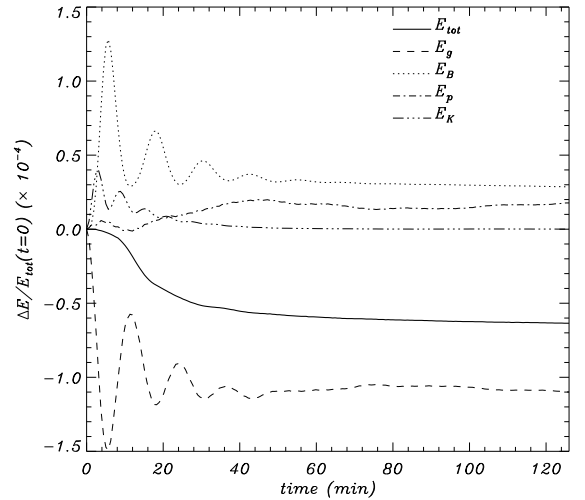
FIG. 8.— Percentage of differences of energies with respect to their values at t = 0 as a function of time. Based on the results of Figure 7.
