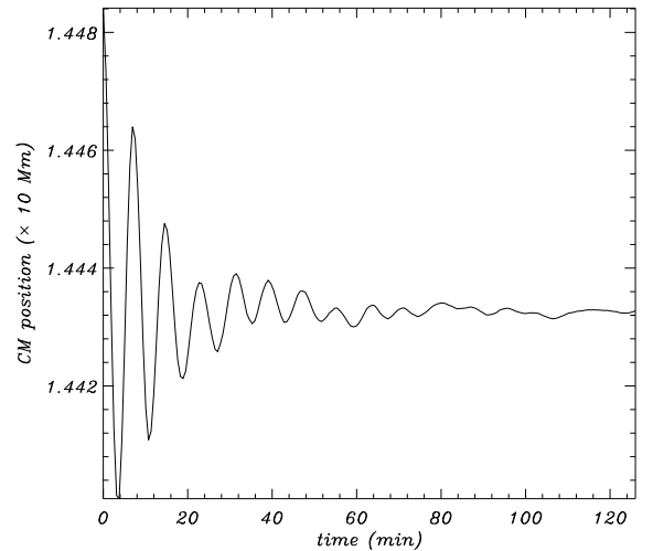
FIG. 10.— Position of the center of mass for the case with a low prominence-corona density contrast. For this case N_t = 2.2 , and the resolution is 600 km.
