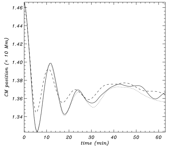
FIG. 5.— Position of the center of mass for three different grid resolutions, 1200 km (dashed line), 600 km (dotted line) and 300 km (continuous line). For this case N_t = 8.5 .
