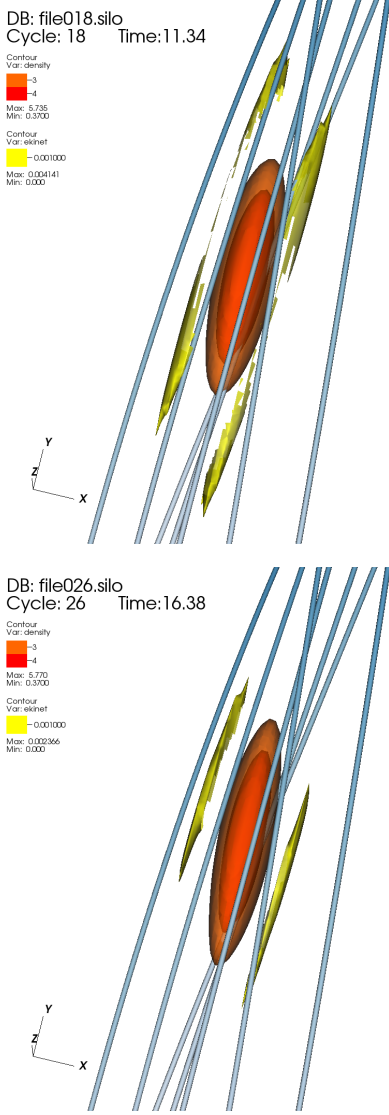
FIG. 11.— Detail of the prominence (red-orange colors) with some magnetic field lines and the locations where the kinetic energy increases (yellow colors) due to continuum damping. For this case N_t = 2.2 . See movie in the online version of the journal.
