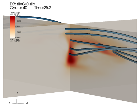
FIG. 17.— Same as in Figure 14 but for N_t = 8.5 .
