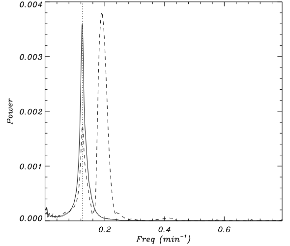
FIG. 12.— Power spectrum of the vertical velocity component at two different positions. The continuous line corresponds to the point close to the center of the prominence while the dashed line is in the PCTR. The two power spectra show a common peak (plotted with a vertical dotted line), associated to the global motion of the prominence (quasi-mode).
