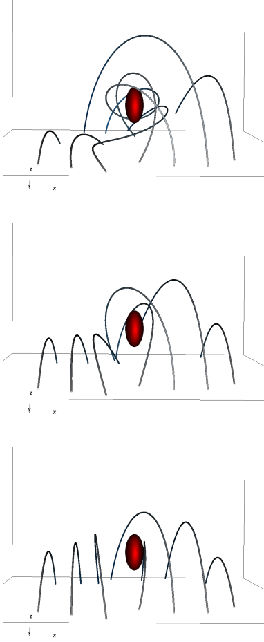
FIG. 1.— Magnetic field configuration and initial density enhancement (in red colors) for N_t = 8.5 (top panel), N_t = 4.3 (middle panel), and N_t = 2.2 (bottom panel). The same magnetic field lines rooted at the base of the corona have been selected in the three plots.
