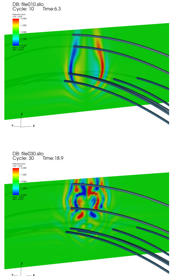
FIG. 13.— Detail of the y -component of the vorticity ( \nabla \times \mathbf{v} ) in the plane y = 0 . For this case N_t = 2.2 and the spatial resolution is 300 km.
