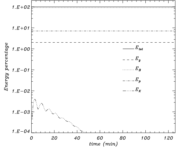
FIG. 7.— Total energies as a function of time. Note the logarithmic scale in the vertical axis. In this simulation the resolution is 600 km and N_t = 2.2 .
