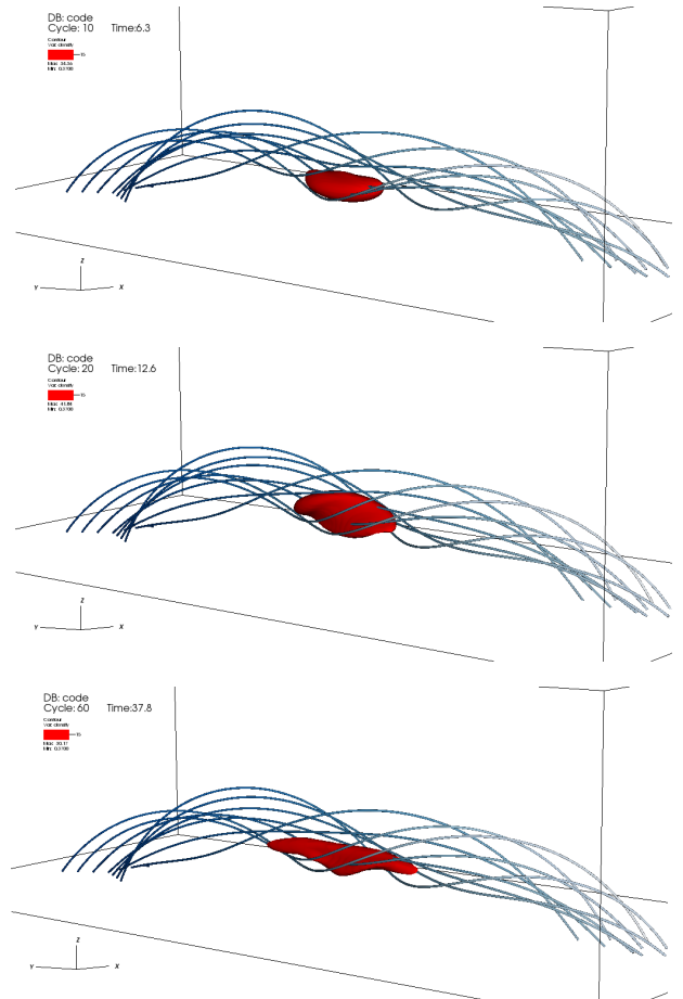
FIG. 3.— Snapshots of the flux rope configuration plus the prominence at three different times. For this case N_t = 8.5 , and the spatial resolution is 600 km. See movie in the online version of the journal.
