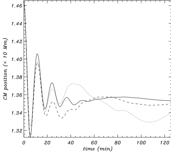
FIG. 6.— Position of the center of mass for three different values of the twist, N_t = 8.5 (dotted line), 4.3 (dashed line), 2.2 (continuous line). In these simulations the resolution is 600 km.
