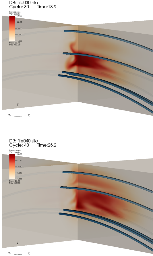
FIG. 14.— Detail of the density evolution at two perpendicular planes. For this case N_t = 2.2 and the spatial resolution is 300 km.
